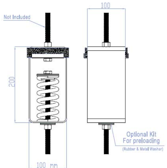
Sides View
