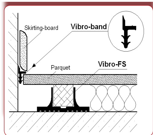
Section view of a parquet antivibration solution
